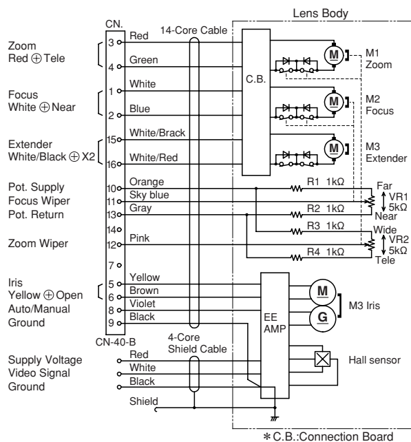
TYPE 5 (DC12V)
