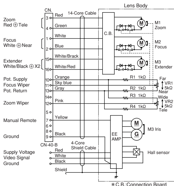
TYPE 5 (DC12V)
