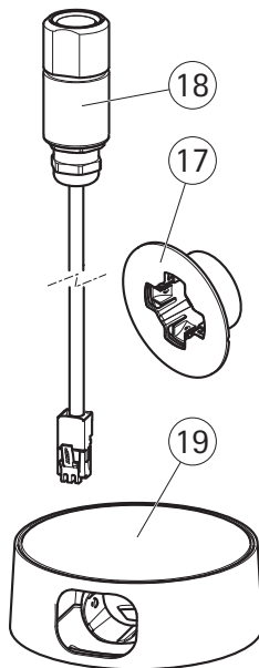
AXIS P1214-E sensor unit and included accessories
