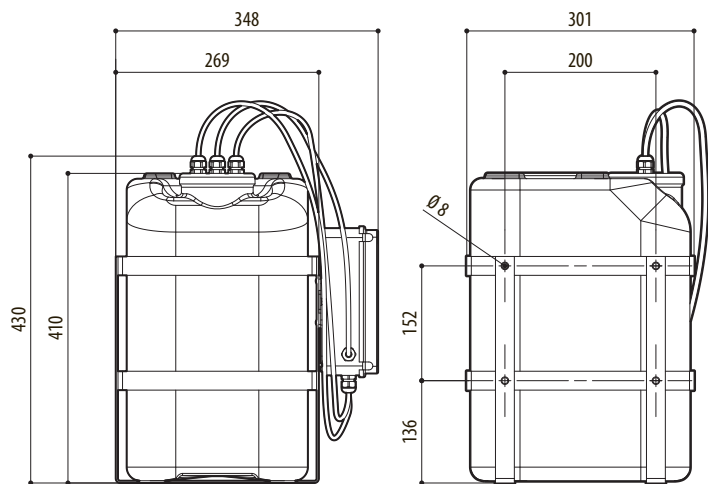
Fig. 50 Water tank 23l (6gal), 11m (36ft) delivery.
