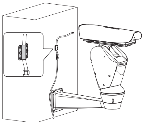
Fig. 45 Example of washer installation on wall.
