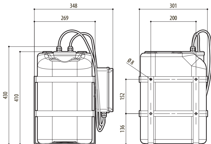
Fig. 49 Water tank 23l (6gal), 5m (16ft) delivery.
