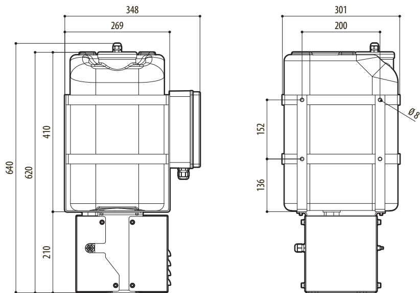
Fig. 51 Water tank 23l (6gal), 30m (98ft) delivery.
