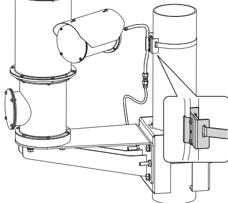
Fig. 46 Example of washer installation on pole.
