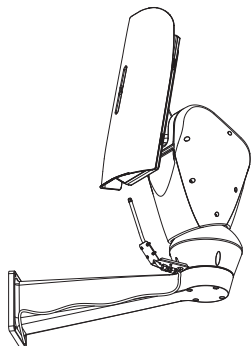
Fig. 44 Example of washer installation on the PTZ camera.
